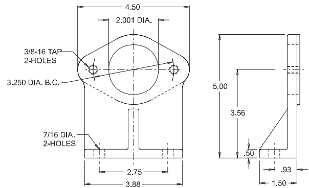
Vescor Part Number Description FM150 SAE AA 2-Bolt Foot Bracket
