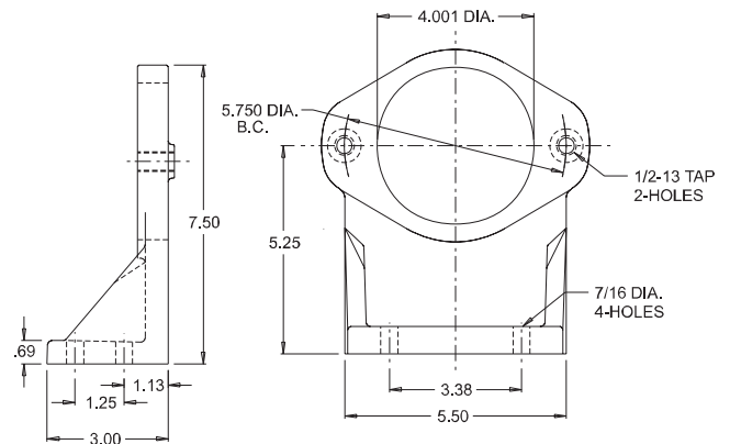
Vescor Part Number Description FM300 SAE B 2-Bolt Foot Bracket
