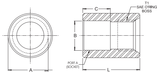
SAE/SOCKET WELD COUPLING
